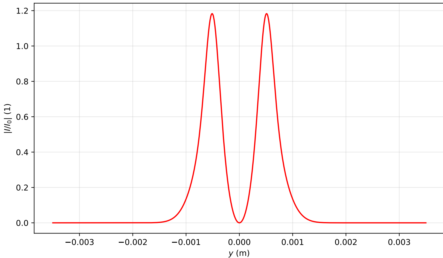
Intensity profile I(x=0, y, z=0.398)/I_0 , P_{in}=6.0P_{cr} , artificial time
